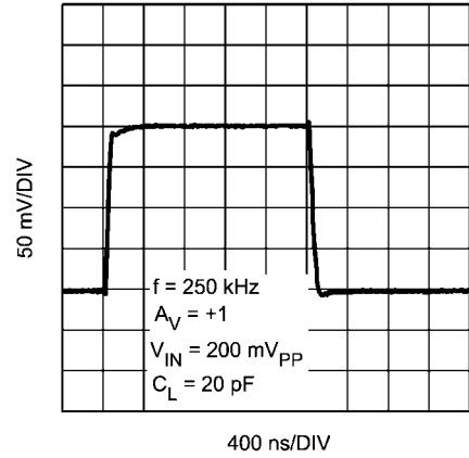
Small Signal Step Response with Gain = 1
